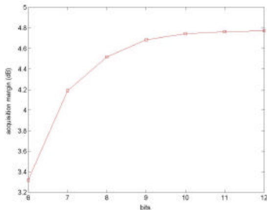
Figure 10: Acquisition margin vs. FFT bit depth for 25-29dB-Hz signals, 10/10 integration, 2000 runs averaged.
