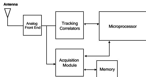
Figure 9: System Block Diagram
