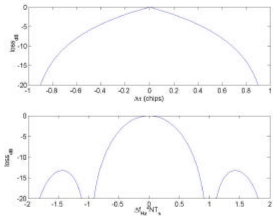
Figure 3: Ambiguity function cross-sections. Top with \Delta\omega=0 , bottom with \Delta\tau=0 .
