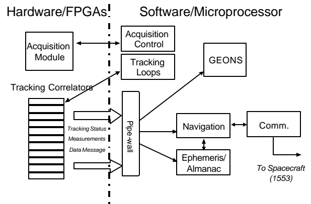
Figure 13: The Navigator software and its interface to the hardware.
