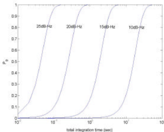
Figure 5: P_D vs. total integration time for 10/M integrations with (\omega, \tau) known and P_{\text{FA}}=0.05/1023
