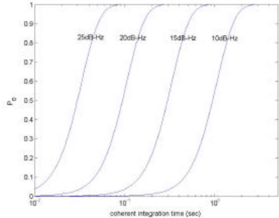
Figure 4: P_D vs. coherent integration time (\omega, \tau) known and P_{\text{FA}}=0.05/1023
