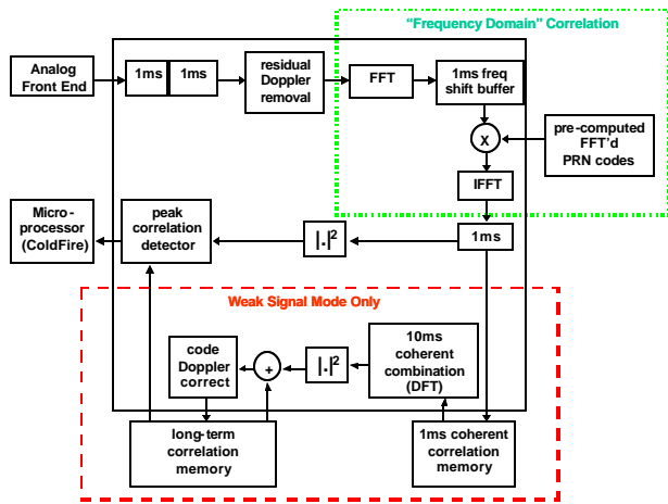
Figure 11: Dual mode acquisition block diagram
