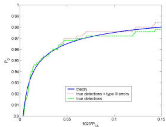
Figure 6: ROC for 10/10 integration, 25dB-Hz signal \omega = 0 known, \tau unknown, P_{\text{FA}} divided down by 1023
