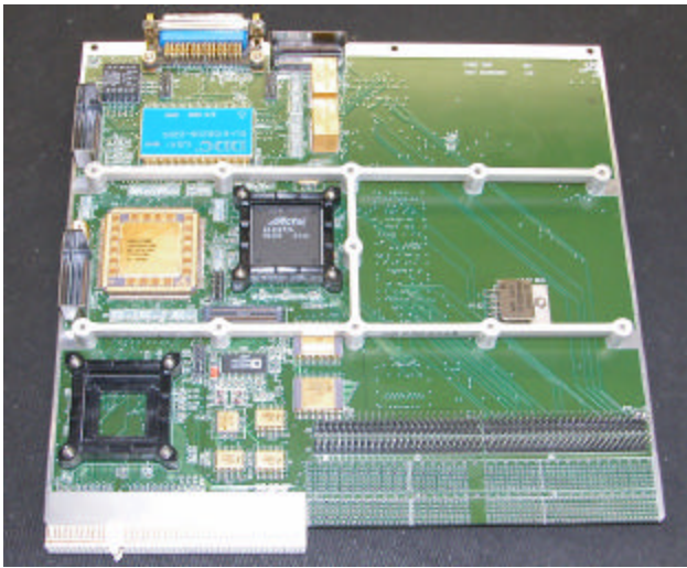
Figure 12: Core SDN, right half will host the GPS specific hardware in the Navigator flight design.
