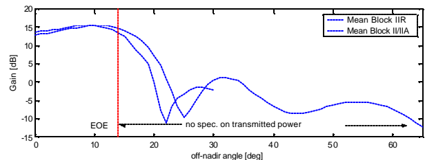
Figure 11: Mean gain patterns for the GPS Block II/IIA [11] and Block IIR [5] satellites.
