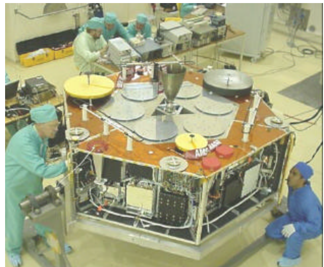
Figure 1: AO-40 spacecraft in Kourou.
