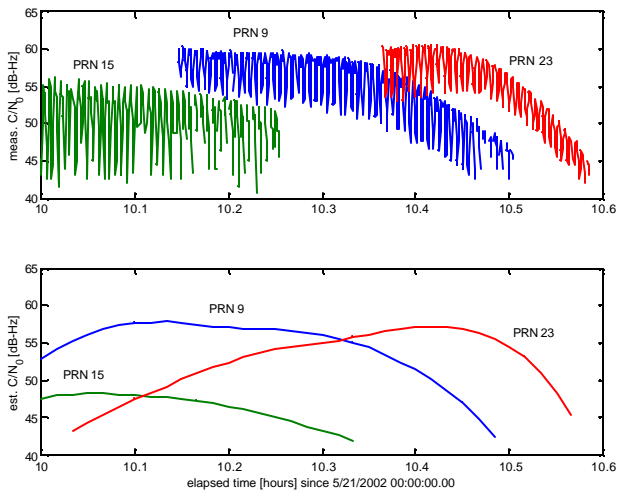
Figure 10: Typical signal levels measured by master antenna near perigee.
