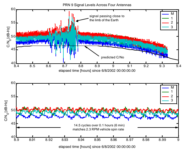
Figure 8: Comparison of signal levels measured from the master and three slave antennas. The top shows a one hour span. The bottom graph shows details over a six minute period. The oscillation in the measurements is due primarily to the spin of the vehicle.
