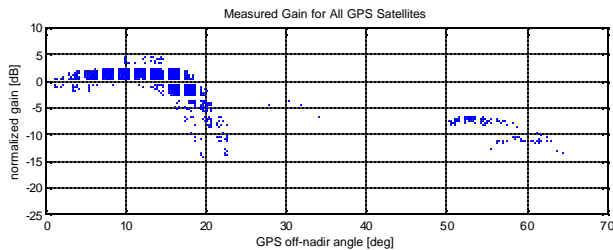
Figure 13: The measured gain pattern of the GPS satellites reconstructed from signal to noise ratio measurements made between 11 May to 15 June 2002.
