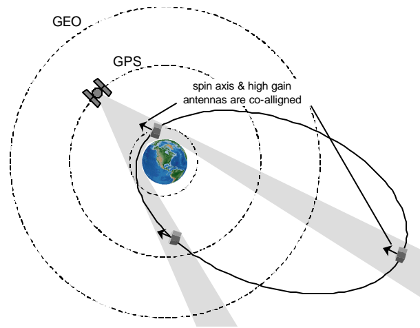
Figure 2: AO-40 orbit and spin axis orientation.
