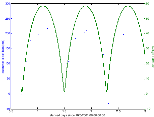
Figure 15: Simulated behavior of the TANS Vector clock in the AO-40 orbit based on a clock drift of 450 m/s.
