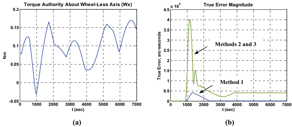
Figure 7 (a) TAWX, (b) Attitude Error
