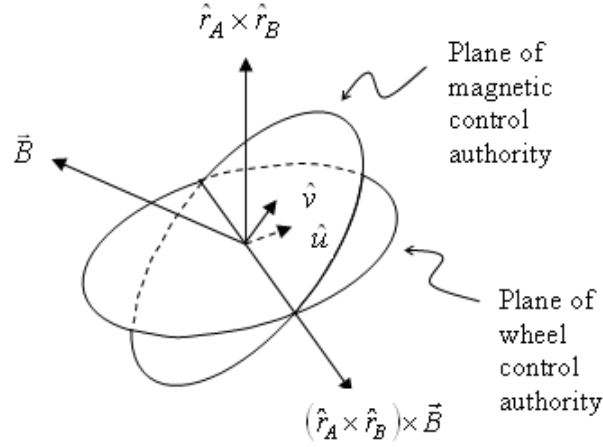
Figure 6 UVN Coordinate Frame
