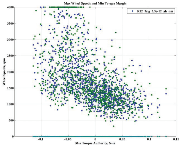
Figure 10 Maximum Wheel Speeds
