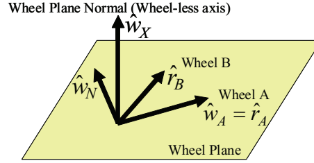
Figure 4 Wheel-Orthogonal-Frame (WOF)
