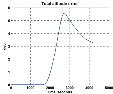
Figure 13 Attitude error corresponding to the case shown in Figure 12
