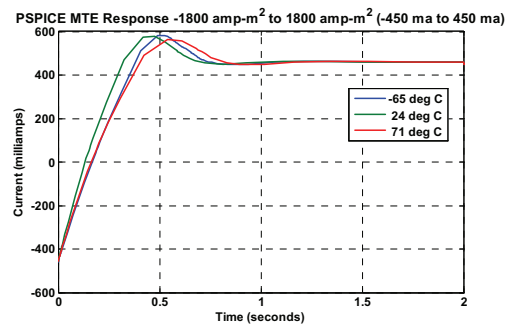
Figure 3 Magnetic Torquer Electronics Time Response
