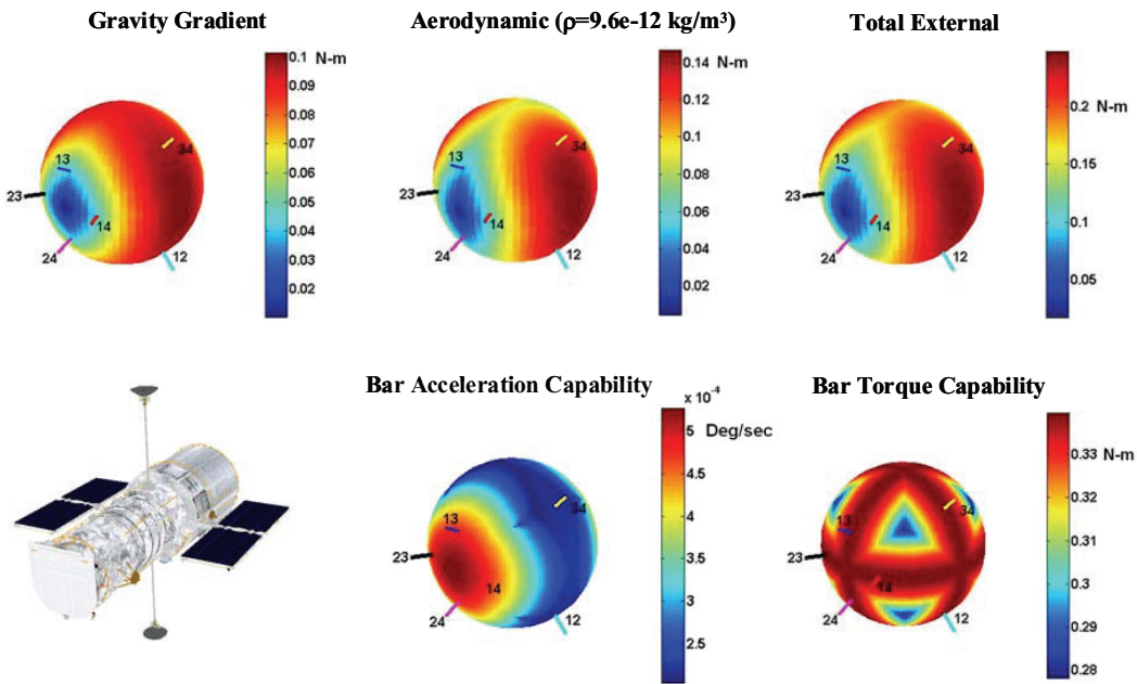
Figure 2 External torque and MTB capability distribution
