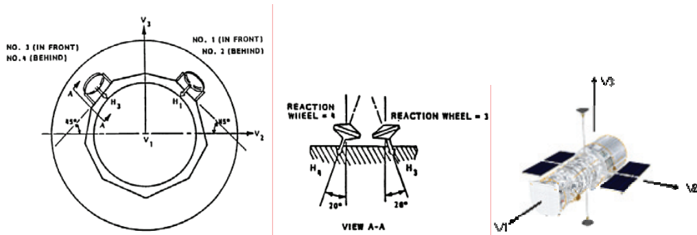
Figure 1 Reaction wheel assembly configuration
