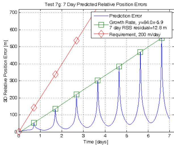
Figure 13: Relative Predictive Position Errors for Phase 1
