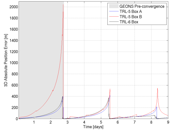
Figure 14: Absolute Position Errors Phase 2
