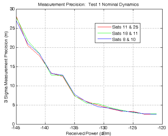
Figure 5: Measurement Noise Test Results
