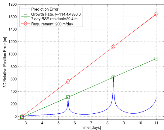
Figure 17: Relative Definitive Errors DUT-TRL-5 Box A Phase 2
