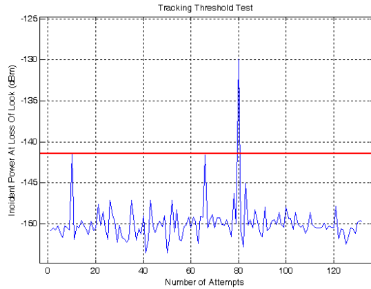
Figure 6: DUT Tracking Threshold Results
