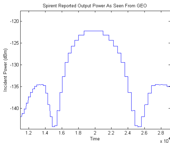
Figure 7: Jumps in the Simulator Reported Output
