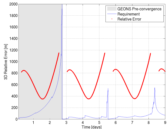
Figure 16: Relative Definitive Errors DUT-TRL-5 Box B Phase 2
