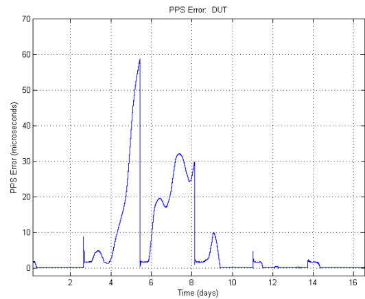
Figure 8: PPS Testing Errors
