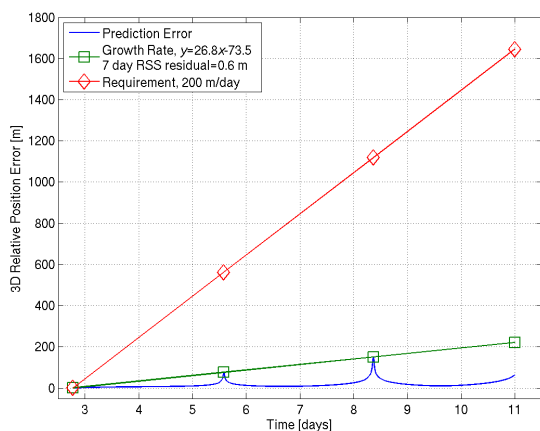
Figure 18: Relative Definitive Errors DUT-TRL-5 Box B Phase 2
