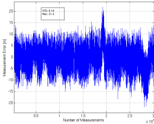
Figure 9: Crosslink Step Test Through Near Mode
