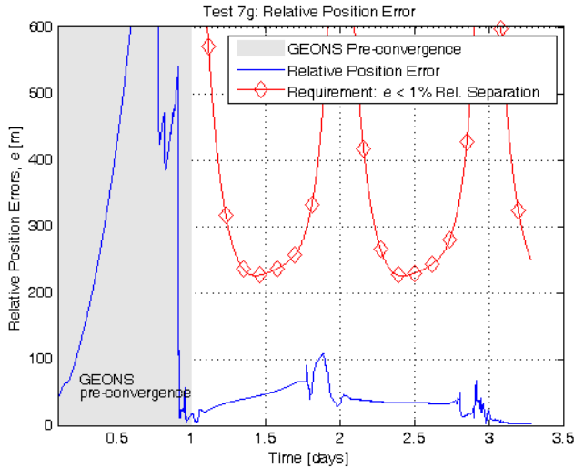
Figure 12: Relative Definitive Position Error for Phase 1
