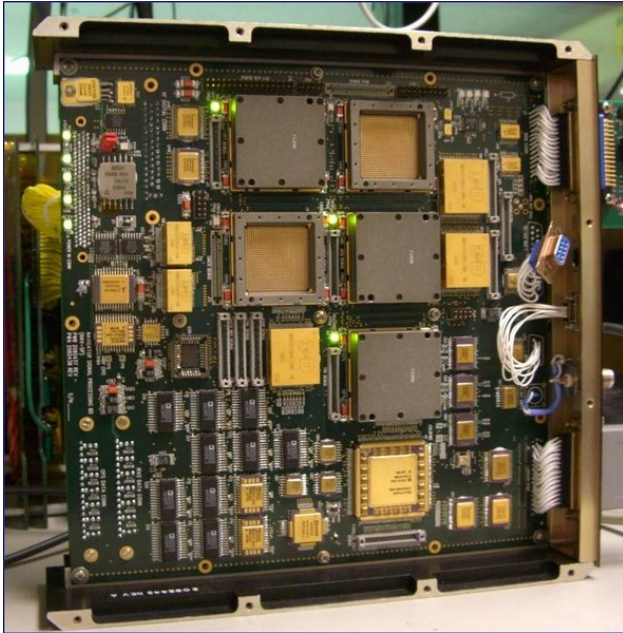
Figure 3: IRAS DUT
