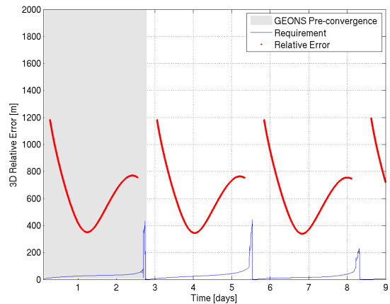
Figure 15: Relative Definitive Errors DUT-TRL-5 Box A Phase 2
