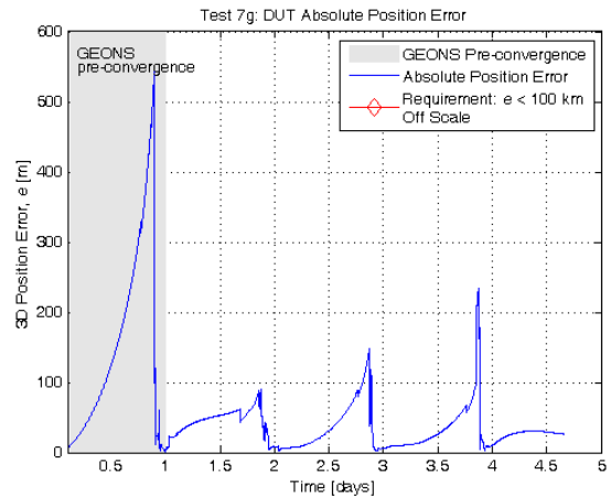
Figure 11: Absolute Position Error for Phase 1
