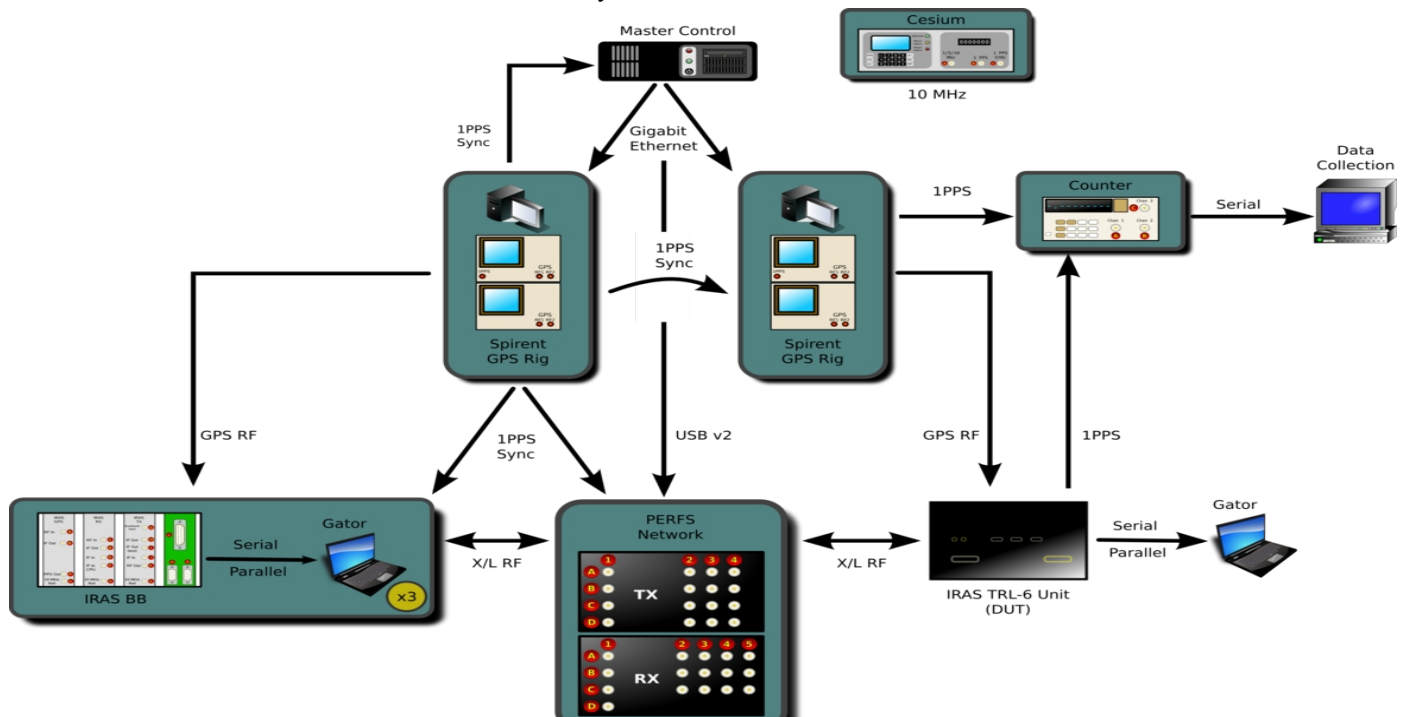
Figure 2: FFTB Laboratory Setup
